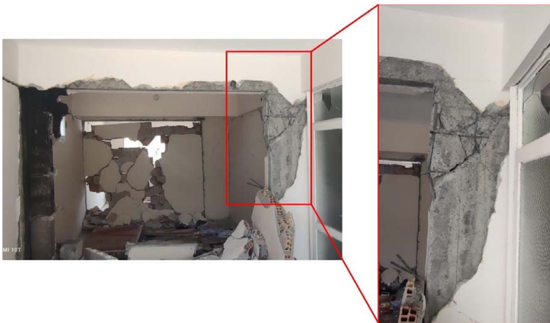
Fig. 5. Brittle shear failure of a r.c. column due to interaction with infills.
